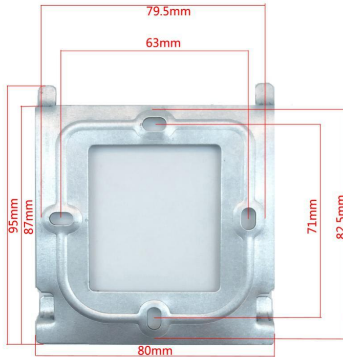
Figure 3-1 Wall Mounting Plate
