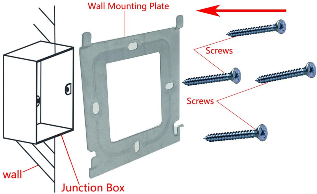
Figure 3-2 Installing the Plate
