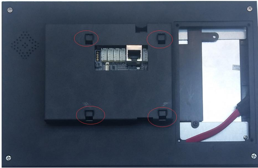
Figure 3-3 Hooking the Indoor Master Station to the Plate
